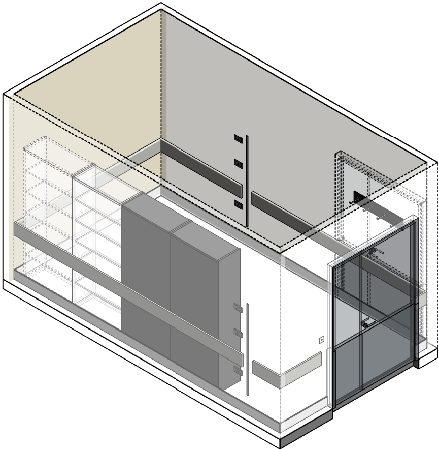
ISOMETRIC VIEW 02
