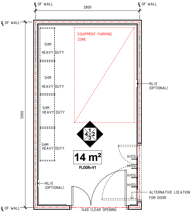
PLAN
