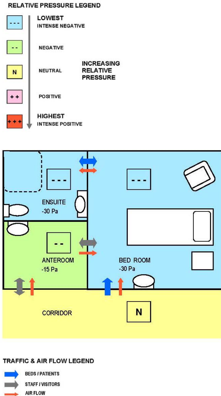
Figure 17: Typical Negative Pressure Isolation Room with Anteroom & Ensuite, showing airflows and relative pressure gradients
