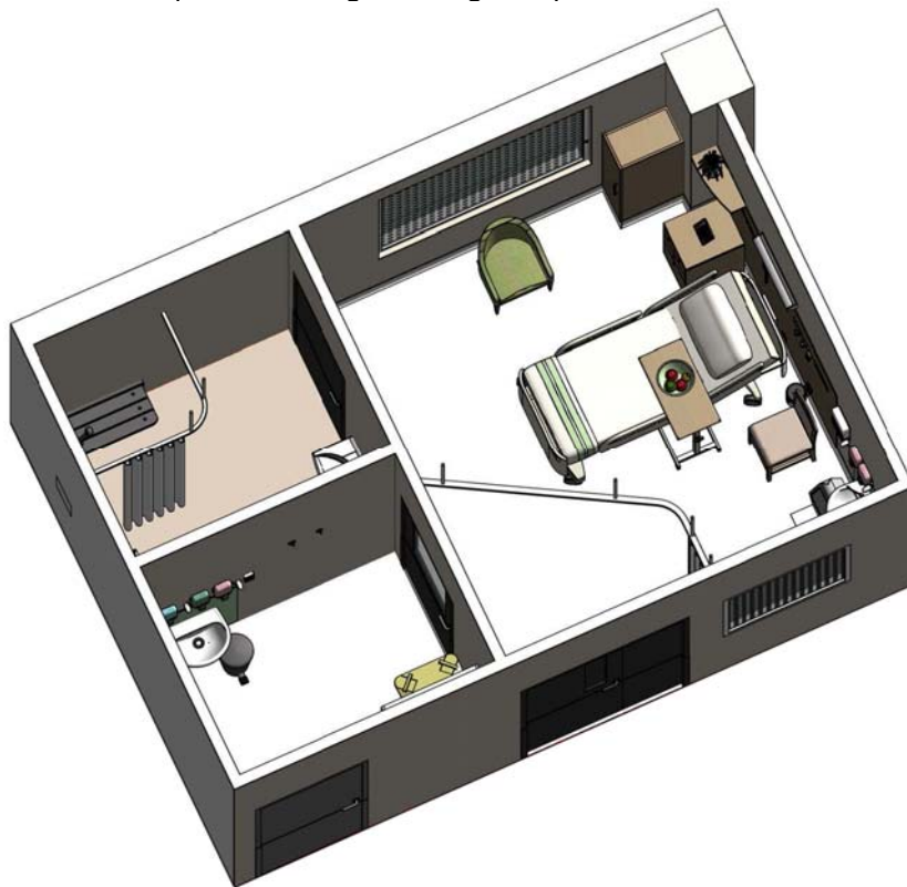
Figure 18: Negative Pressure Isolation room including Ensuite and Anteroom
