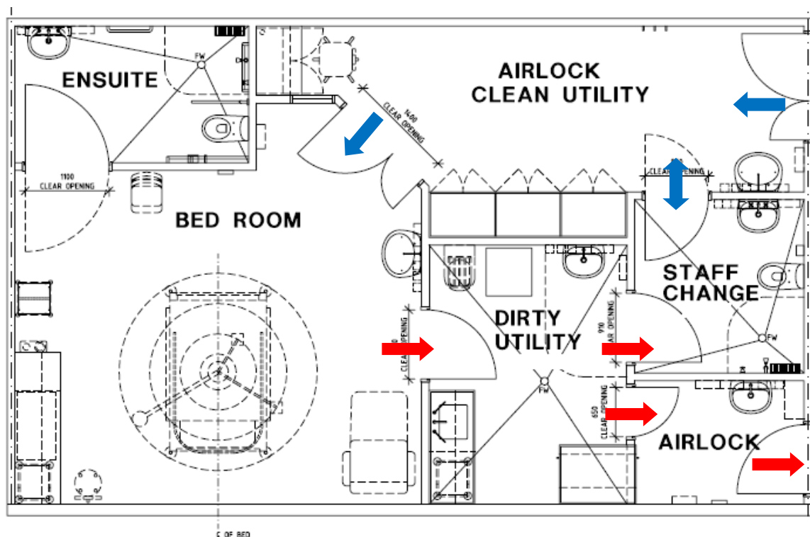
Figure 19: Typical plan of Class Q Quarantine Suite.
