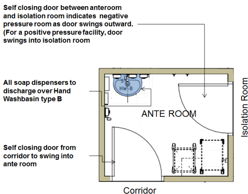
Figure 16: Typical Anteroom plan
