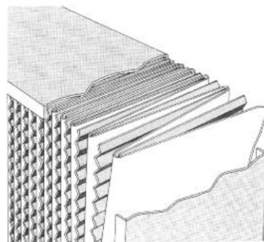
Typical HEPA filter construction
